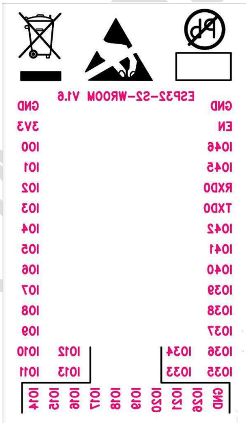
ESP32-S2-WROOM ESP32-S2-WROOM-I
