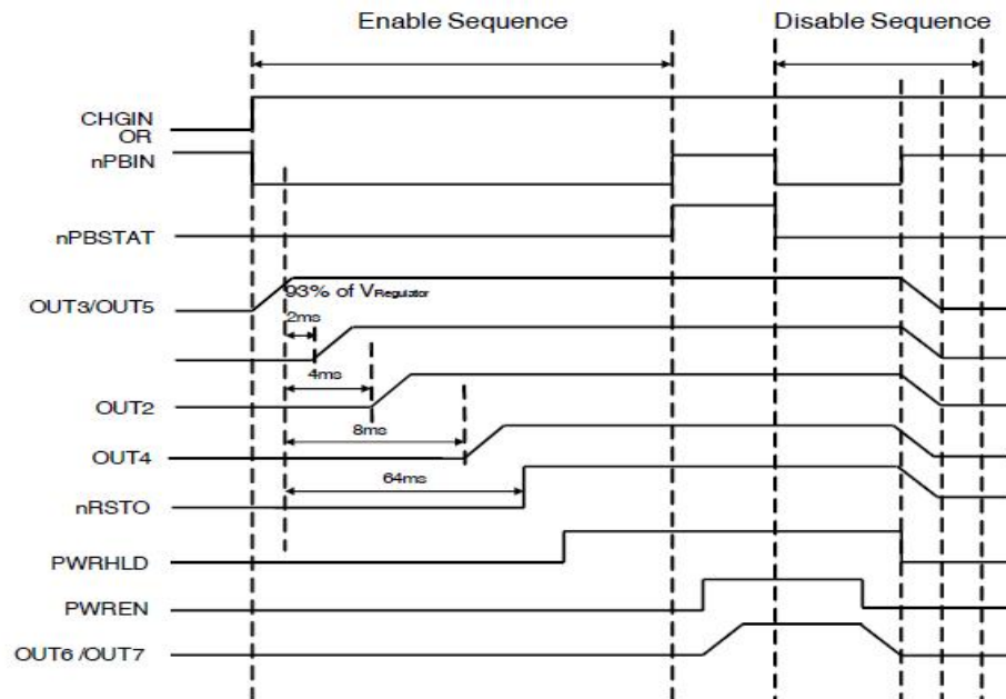
ACT8945AQJ305-T Enable/Disable Sequence
