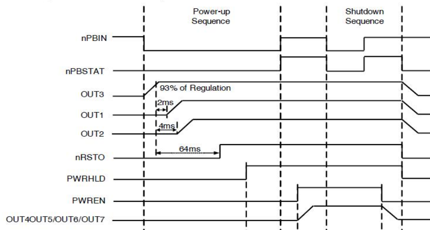
ACT8945AQJ303-T Enable/Disable Sequence
