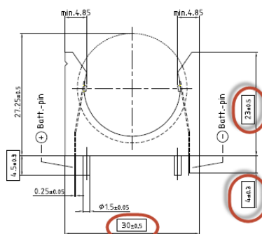
adjusted drawing 3.8755.4-2 according real production
