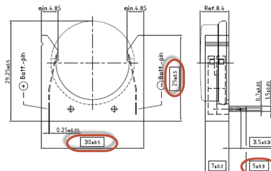
adjusted drawing 3.8755.4-2 according real production
